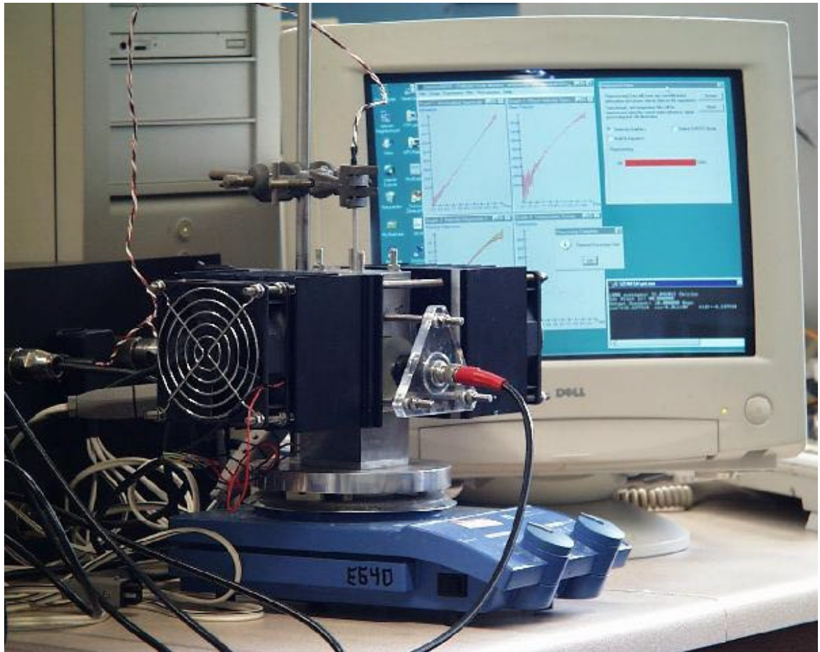
Figure B.3: Temperature controller and batch crystallizer test-cell for monitoring of copper sulphate pentahydrate crystallization.
