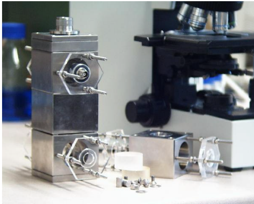
Figure B.2: Illustration of modular test-cell with two vertically displaced test positions.
