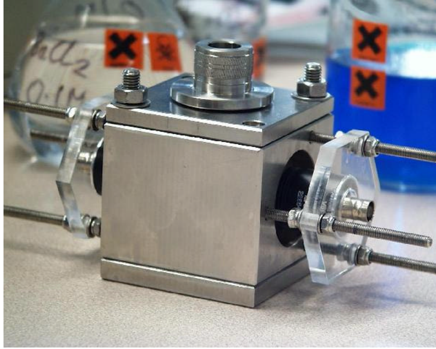
Figure B.1: Stainless steel (S316) ultrasonic test-cell in pulse transmission configuration.
